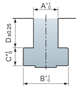
T-Slot Dimensions
