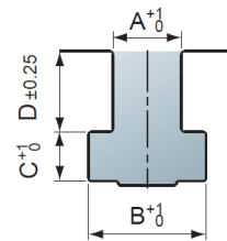
T-Slot Dimensions
